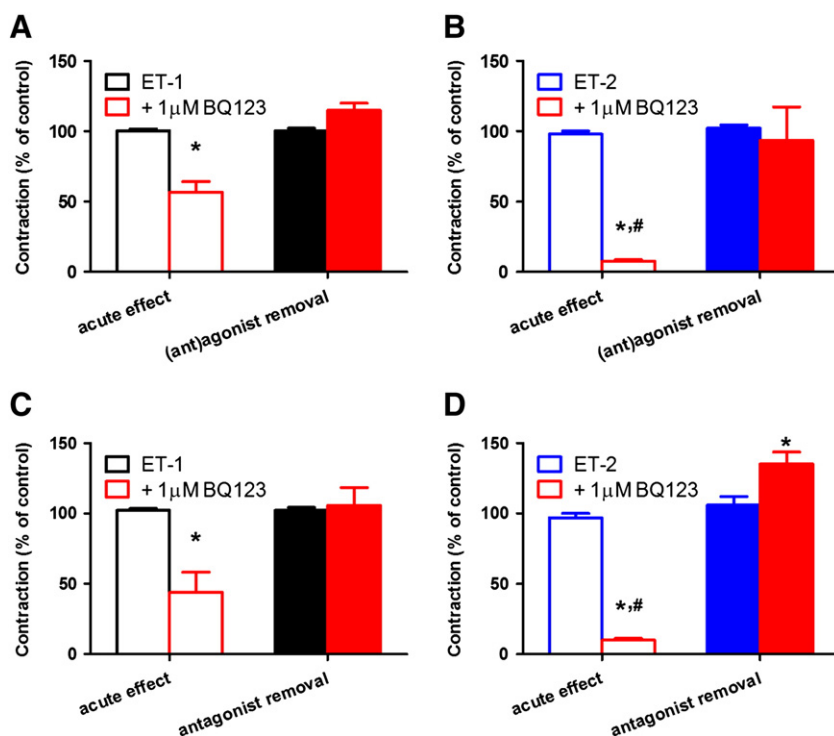
Fig. 2. Inhibitory effects of BQ123 on sustained and maintained contractions. 1 \mu M BQ123 reduces ET-1-induced contractions by approximately 50% in presence (A) or following removal (C) of free agonist. The BQ123-induced inhibitions were rapidly reversed upon removal of antagonist and/or agonist. ET-2-induced contractions were reduced by 1 \mu M BQ123 by approximately 90% in presence (B) or following removal (D) of free agonist. Again, these BQ123-induced inhibitions were rapidly reversed upon removal of the ligand(s). * P < 0.05 vs control, # P < 0.05 vs BQ123 effect on ET-1.
