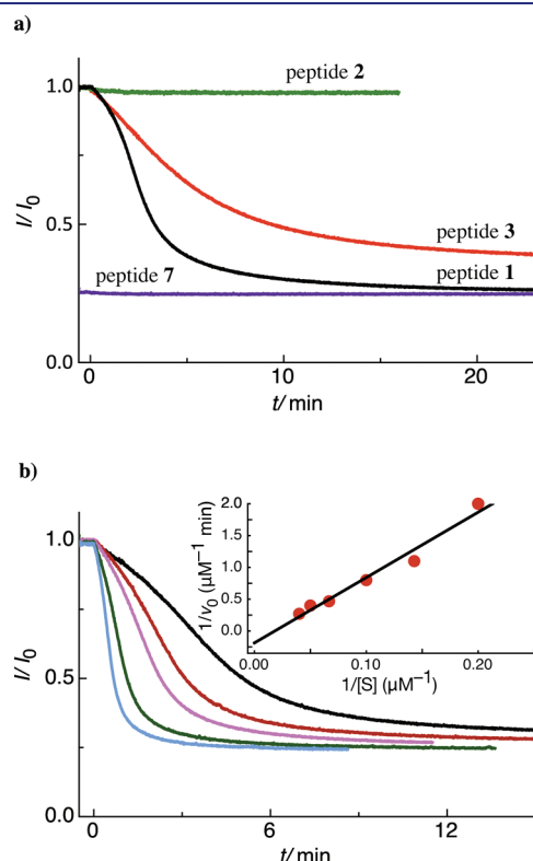
Figure 3. (a) Continuous fluorescence assays ( \lambda_{\text{exc}} = 485 nm, \lambda_{\text{obs}} = 510 nm) with the CB7/AO reporter pair ( 8 \mu\text{M}/0.5 \mu\text{M} ) upon addition of thermolysin ( t = 0 min, 15 nM) to peptides 1–3 and 7 ( 30 \mu\text{M} ), at 37^\circ\text{C} . (b) Determination of enzyme kinetic parameters by monitoring of thermolysin ( 15 nM) activity with varying concentration of enkephalin 1 ( 5 – 25 \mu\text{M} ) in 10 mM ammonium phosphate buffer, pH 7.2 , at 37^\circ\text{C} with the CB7/AO reporter pair ( 2.5 \mu\text{M}/0.5 \mu\text{M} ). I_0 and I are the fluorescence intensities at time t = 0 and time t , respectively.
