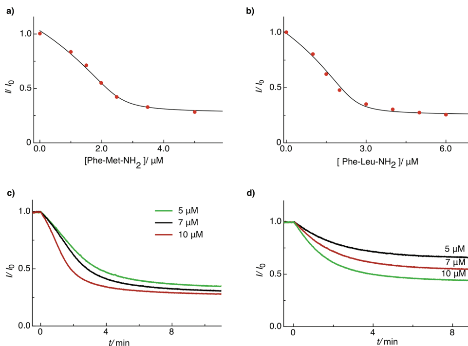
Figure 4. Fluorescence measurements using CB7/AO (2.5 \mu\text{M} CB7 and 0.5 \mu\text{M} AO, \lambda_{\text{exc}} = 485 \text{ nm} , \lambda_{\text{obs}} = 510 \text{ nm} ) as a reporter pair in 10 mM ammonium phosphate buffer, pH 7.2, at 37 ^{\circ}\text{C} . Competitive fluorescence titration plots of (a) Phe-Met-NH 2 (7) and (b) Phe-Leu-NH 2 (8). Tandem protease assays for thermolysin (15 nM) with substrates (c) Thr-Gly-Ala-Phe-Met-NH 2 (1) and (d) Thr-Gly-Ala-Phe-Leu-NH 2 (3).
