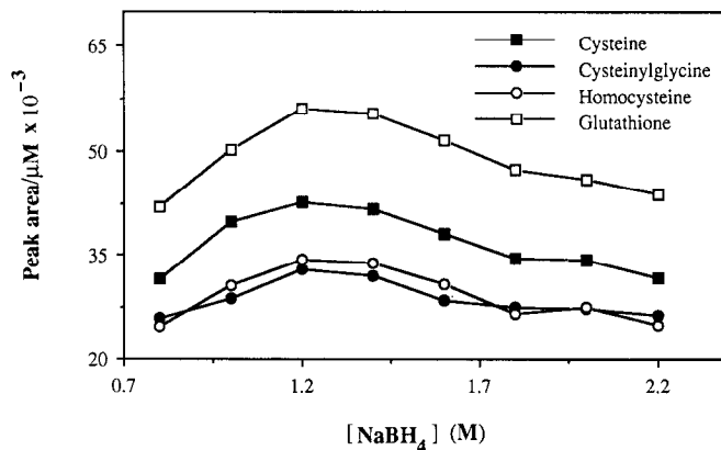
FIG. 2. The effect of the concentration of \text{NaBH}_4 on the reduction of a standard solution containing the disulfide forms of cysteine (100 \mu\text{M} ), cysteinylglycine (12.5 \mu\text{M} ), homocysteine (5 \mu\text{M} ), and glutathione (5 \mu\text{M} ). The thiol components were prepared in 5% sulfosalicylic acid/50 \mu\text{M} DTE and pretreated with \text{NaBH}_4 at concentrations indicated and then derivatized with mBrB using procedure 1 (as described under Materials and Method). The concentrations of \text{NaBH}_4 refer to the standard solution.
