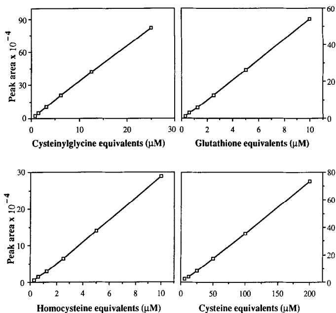
FIG. 4. Standard curves for cysteine, cysteinylglycine, homocysteine, and glutathione. The standards were dissolved in 5% sulfosalicylic acid containing 50 \mu\text{M} DTE. Samples were analyzed by procedure 1.
