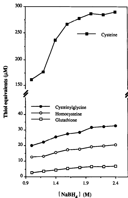
FIG. 3. The effect of the concentration of \text{NaBH}_4 on the yield of cysteine, cysteinylglycine, homocysteine, and glutathione from plasma. Plasma was pretreated with \text{NaBH}_4 at the concentrations indicated (refers to the standard solution) and then derivatized with mBrB using procedure 1.
