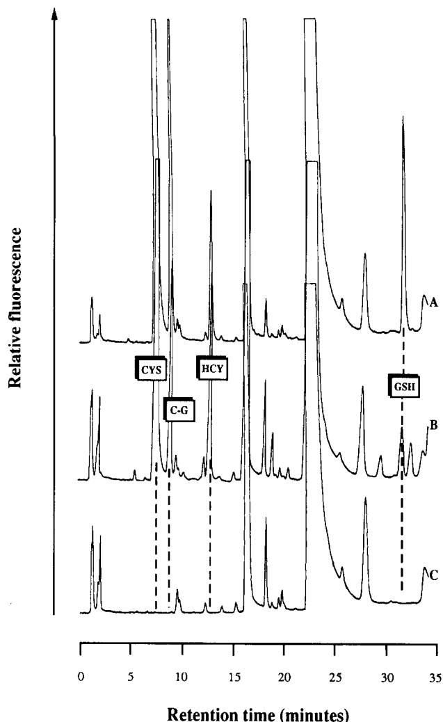
FIG. 1. Reversed-phase high-performance liquid chromatogram of a mBrB-derivatized sample of (A) standard solution composed of 200 \mu\text{M} cysteine (CYS), 25 \mu\text{M} cysteinylglycine (C-G), 10 \mu\text{M} homocysteine (HCY), and 10 \mu\text{M} glutathione (GSH) in 5% sulfosalicylic acid/50 \mu\text{M} DTE; (B) whole plasma (total thiol components); and (C) 5% sulfosalicylic acid/50 \mu\text{M} DTE (blank). Procedure 1 was used as described under Materials and Methods.
