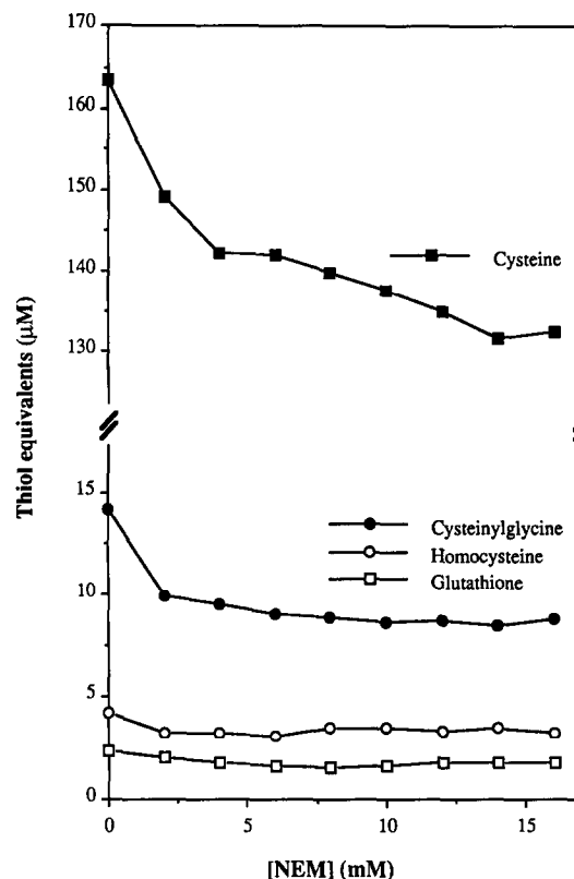
FIG. 9. Determination of the optimal NEM concentration needed to block sulfhydryl groups in human plasma. NEM solutions of varying concentrations were prepared in PBS and 500 \mu\text{l} of each solution was injected into 5-ml evacuated blood collection tubes containing heparin. Blood from healthy subjects was drawn and the isolated plasma further treated as described in procedure 2. Final NEM concentrations in the tubes are indicated.
