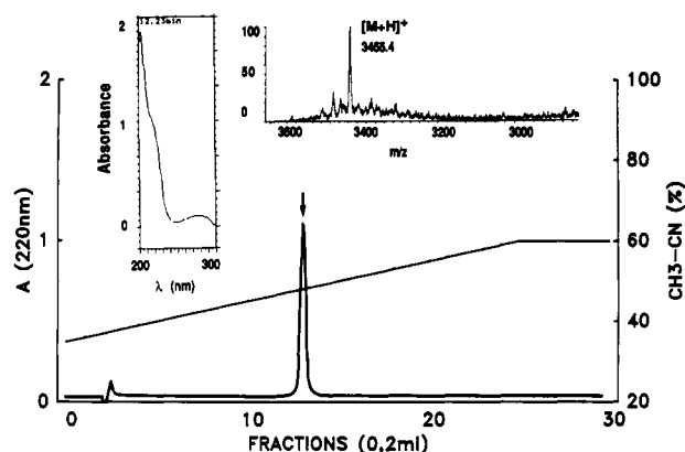
FIGURE 2: Final purification step of dermaseptin, performed on an analytical Delta-Pac (Waters, C18 5 \mu\text{m} , 150 \text{ mm} \times 2 \text{ mm} ) column. Elution was achieved with a linear gradient of 35–60% acetonitrile in 0.1% TFA/water for 25 min at a flow rate of 0.2 mL/min. The arrow points to the elution position of synthetic dermaseptin under the same conditions. The left-hand inset represents the UV absorbance spectrum of the eluting peak at 12.23 min. The right-hand inset represents the quasi-molecular ion region of the positive FAB mass spectrum of purified dermaseptin.
