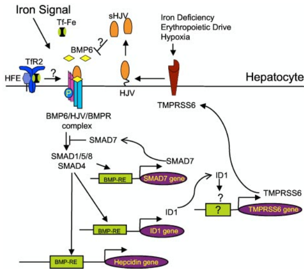
Figure 5. Schematic representation showing proposed role of TMPRSS6 regulation by the BMP6-SMAD signaling pathway and iron via ID1. We propose that, in addition to being stimulated by several signals that inhibit hepcidin, such as iron deficiency, erythropoietic drive, and hypoxia, TMPRSS6 expression is also stimulated indirectly by the hepcidin activators BMP6 and iron. Stimulation by BMP6 and/or iron induces an increase of the BMP6-HJV-SMAD pathway activity, possibly through a mechanism involving HFE and transferrin receptor 2 (TFR2), leading to binding of SMAD complexes to BMP-responsive elements (BMP-REs) on the hepcidin promoter and up-regulation of hepcidin transcription. In parallel, BMP6-SMAD pathway directly up-regulates SMAD7 and ID1 transcription. ID1 induction leads to the up-regulation of TMPRSS6 expression. TMPRSS6 then serves as a negative feedback inhibitor of BMP-SMAD pathway activity and hepcidin expression by cleaving the BMP coreceptor HJV. Inhibitory SMAD7 can also act as a negative feedback inhibitor by blocking SMAD activation. By acting as negative feedback inhibitors, TMPRSS6 and SMAD7 are important to prevent excessive hepcidin increases in response to BMP6 and iron, thereby maintaining tight control of iron homeostasis. Abbreviations: BMPR indicates BMP receptor; TF-Fe, holotransferrin; sHJV, soluble hemojuvelin; and BMP-RE, BMP responsive element.
